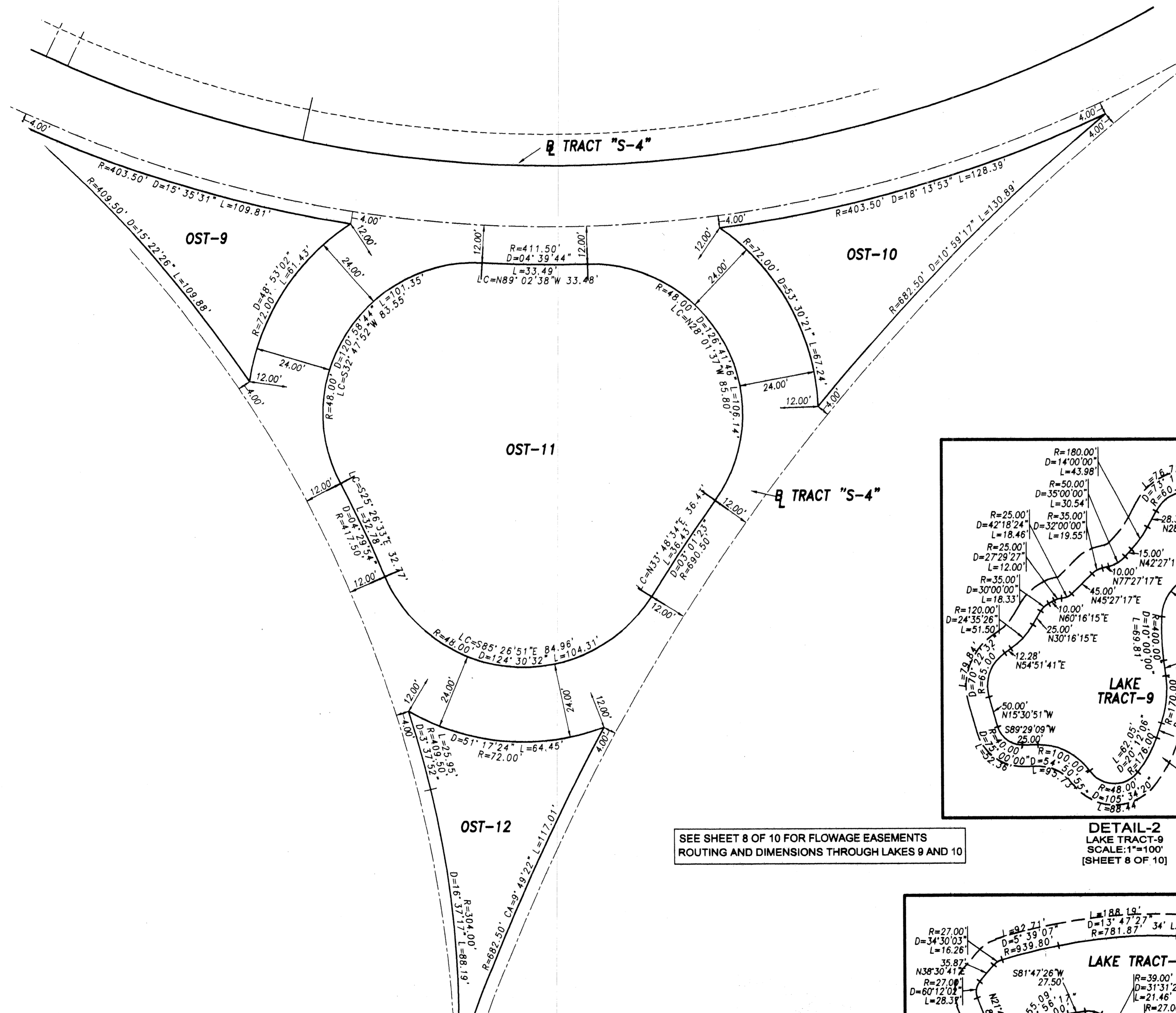
DETAIL-1 OPEN SPACE TRACTS 9, 10, 11, AND 12 SCALE: 1"=20' (SHEET 8 OF 10)
