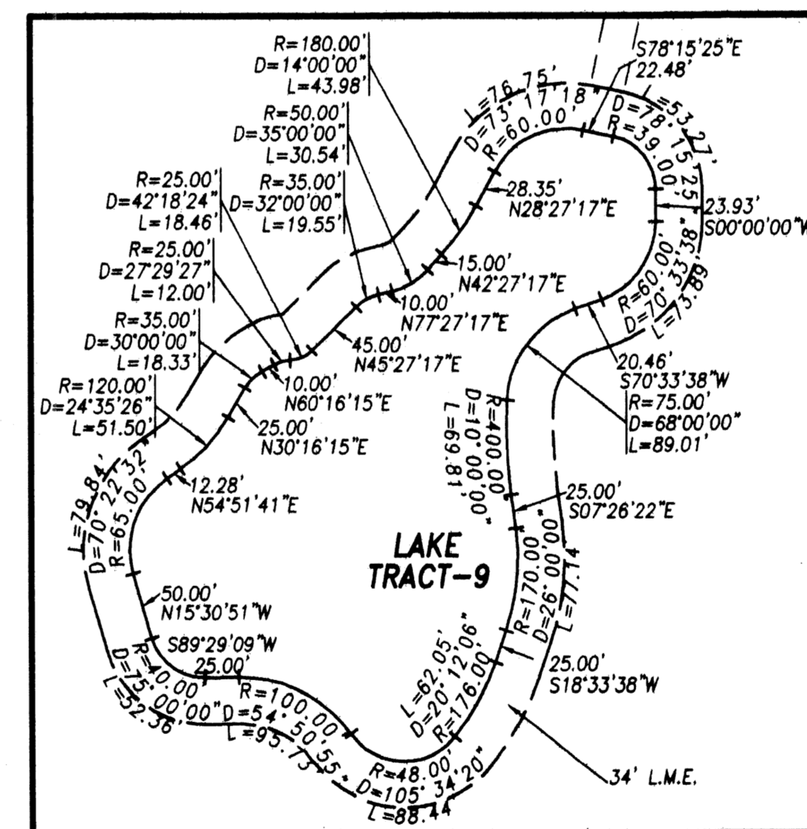
DETAIL-2 LAKE TRACT-9 SCALE: 1"=100' (SHEET 8 OF 10)
