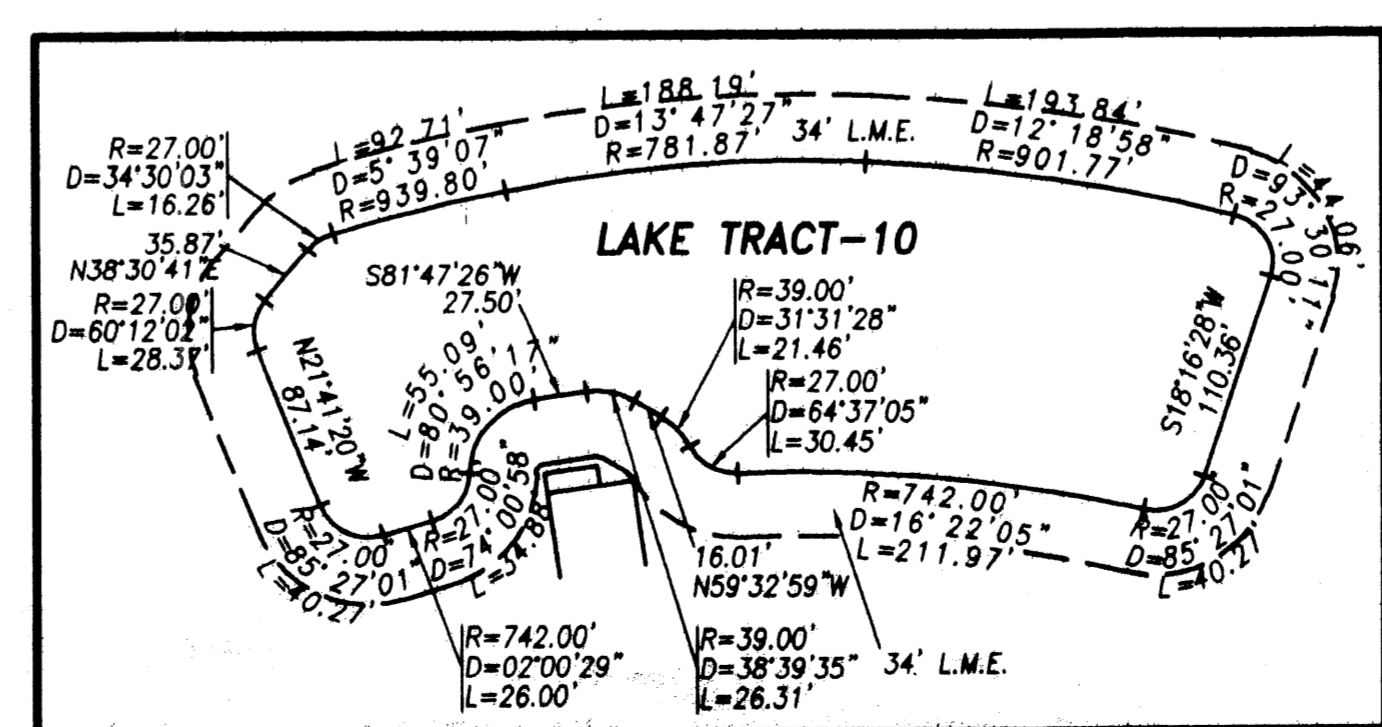
DETAIL-3 LAKE TRACT-10 SCALE: 1"=100' (SHEET 8 OF 10)
